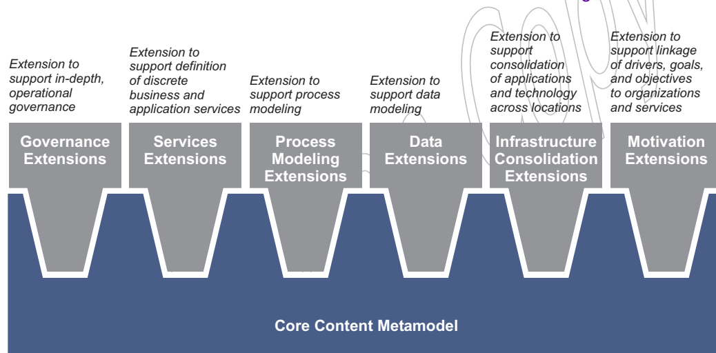
Figure 34-1 TOGAF Content Metamodel and its Extensions
