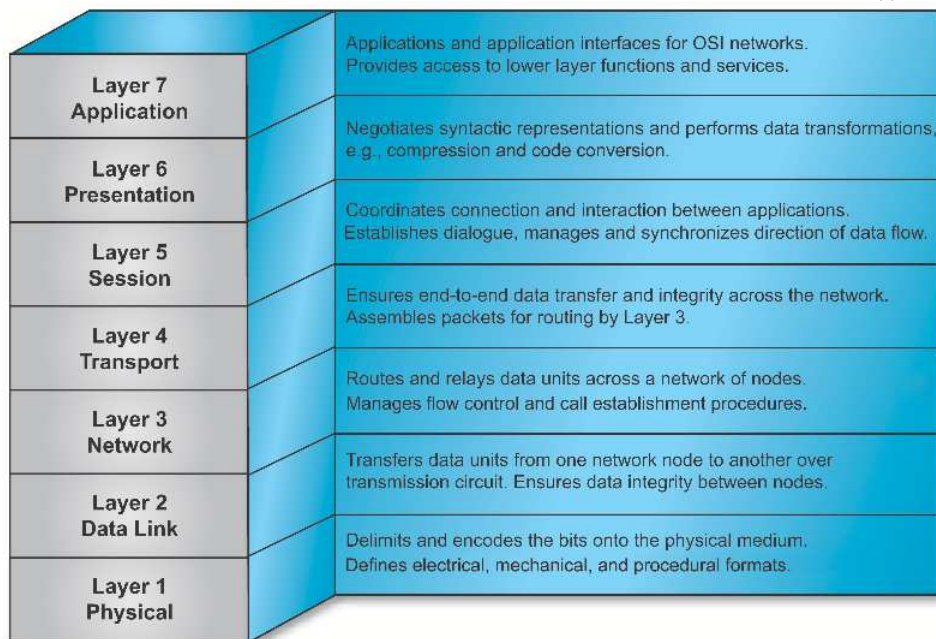
Figure 35-16 OSI Reference Model
