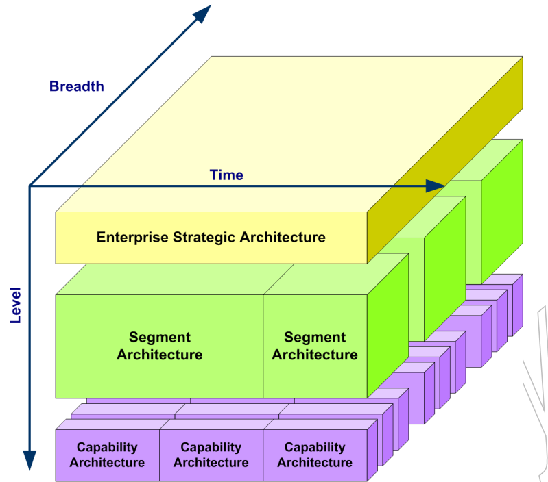
Figure 20-1 Summary Classification Model for Architecture Landscapes
